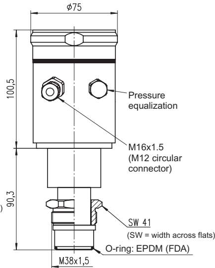
Field housing with integrated display (stainless steel, IP67 EN 60529)
