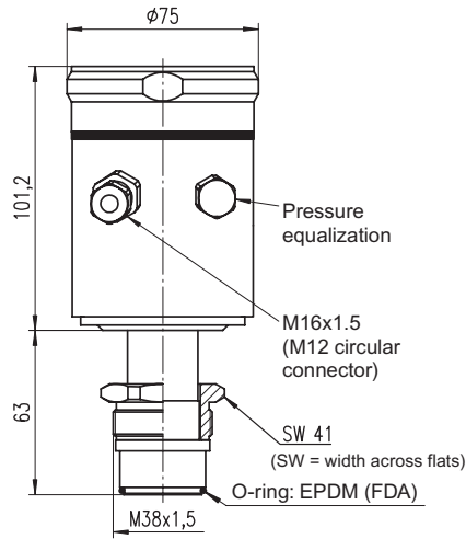
PIEZOMESS 100 ... _K(M)
